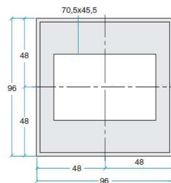
96x96 / 4TE
